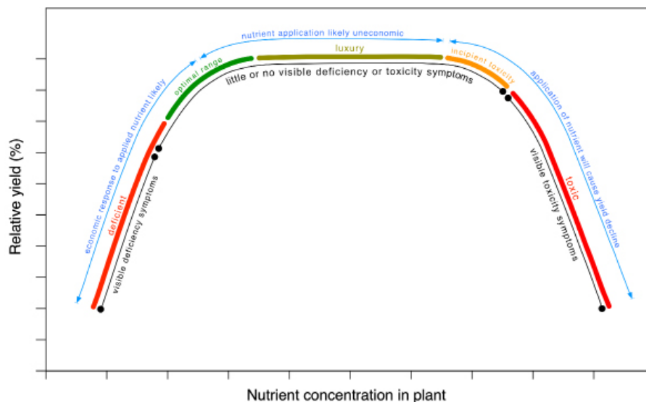
Figure 2-1. General relationship between plant nutrient concentration and relative yield
