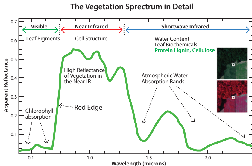
Figure 8-3. Vegetation spectrum details (accessed 05/05/2021, https://www.isharrisgeospatial.com/Learn/Whitepapers/Whitepaper-Detail/ArtMID/17811/ArticleID/16162/Vegetation-Analysis-Using-Vegetation-Indices-in-ENVI )
